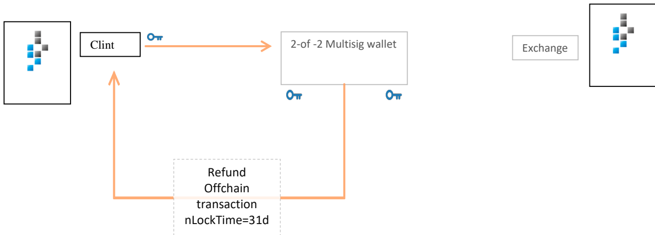
Figure 5: Off the blockchain refund transaction is signed by the exchange. Refund transaction will be valid after 31 days lock.
