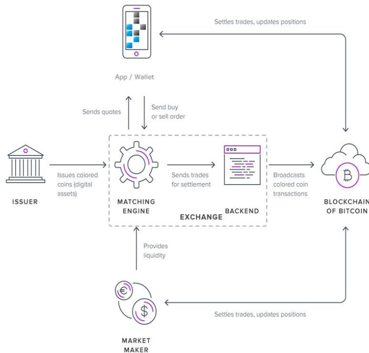
Figure 7: Bits Digit Exchange high-level architecture
