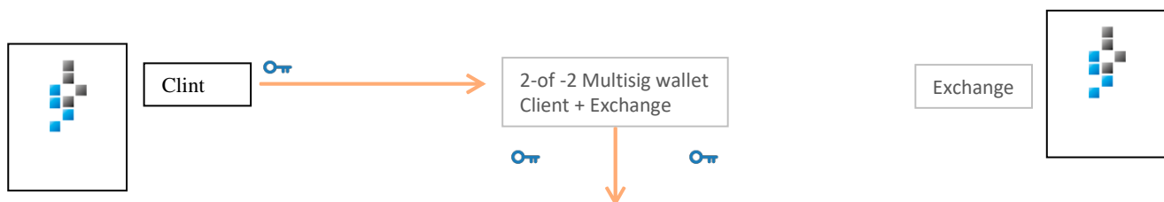
Figure 4: 2-of-2 multisignature address used to deposit trader's coins. Two signatures are required to spend coins – both trader's and exchange's.
