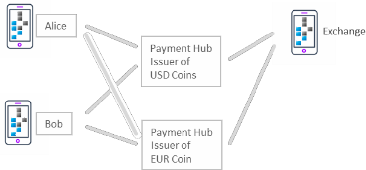
Figure 6: Both exchange and traders have micropayment channels with Payment Hubs to be able to transfer multiple types of coins off the blockchain. Issuer of the coins may act as Payment Hub.
